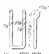
Figs. 4768-4769. Brake-beam Hangers (1).
